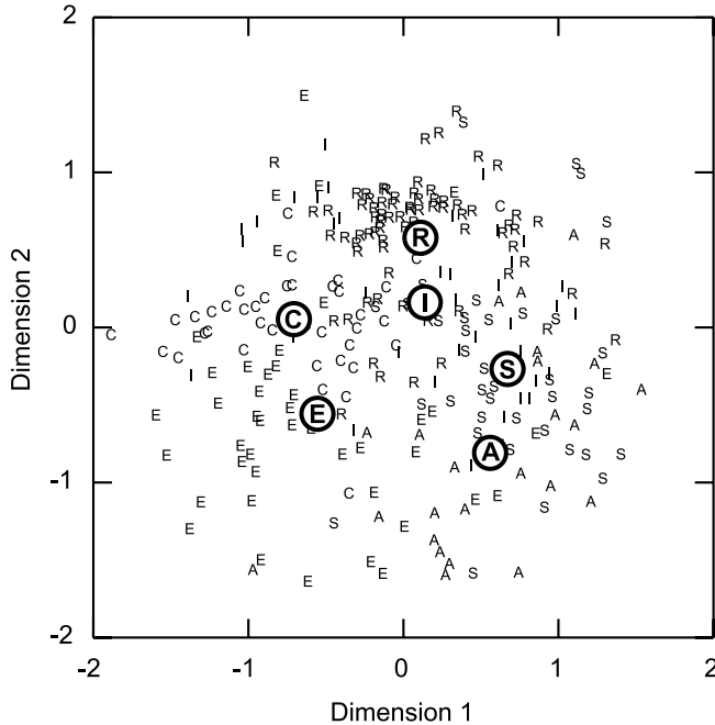
Fig. 2. Two-dimensional MDS configuration of the 268 OPI occupations plotted by first-letter RIASEC code. Centroid coordinates for each RIASEC type are circled.
