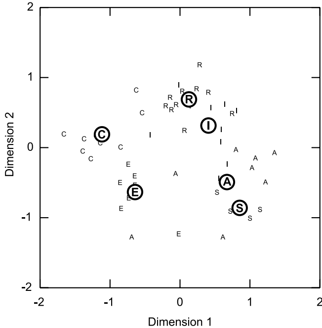
Fig. 4. Two-dimensional MDS configuration of the 49 VPI occupations plotted by first-letter RIASEC code. Centroid coordinates for each RIASEC type are circled.
