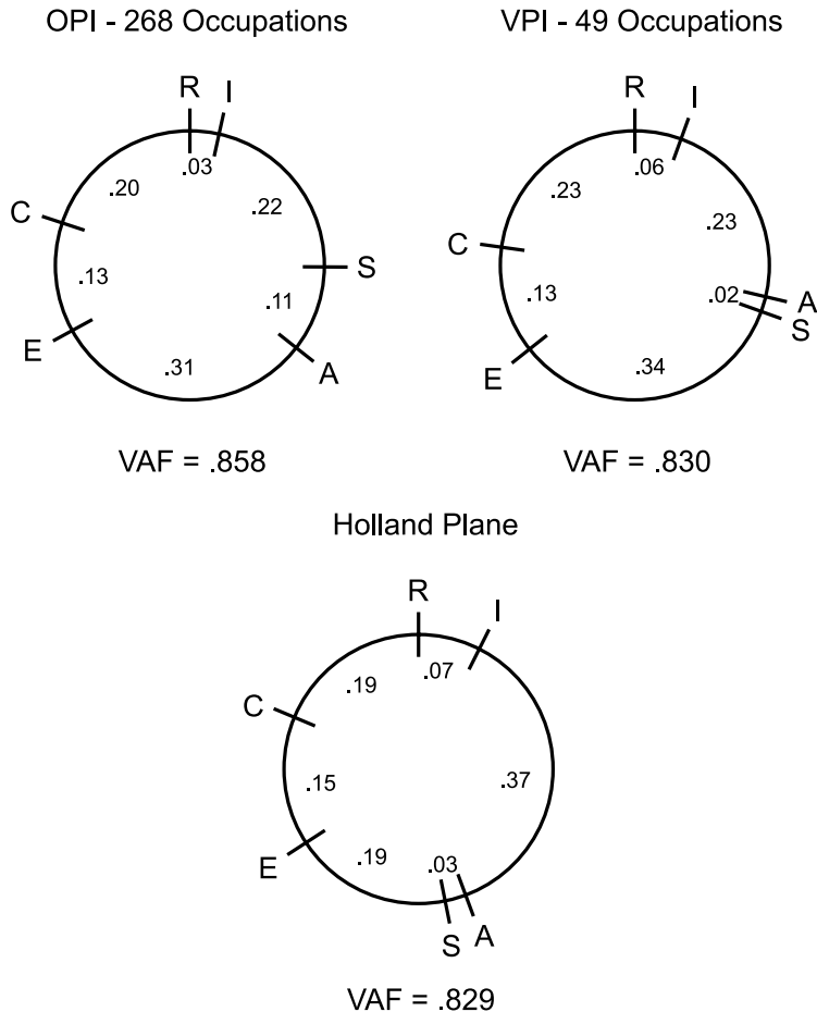
Fig. 3. Circular Unidimensional Scaling results for RIASEC centroids obtained from the two-dimensional MDS solution for 268 OPI and 49 VPI occupations and the Holland Plane of the rotated three-dimensional MDS solution for 268 OPI occupations.
