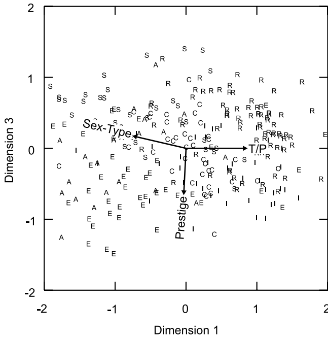
Fig. 6. Property vector fitting results for dimensions one and three of the rotated three-dimensional MDS solution, with occupations plotted by first letter RIASEC code. T/P, Things/People.
