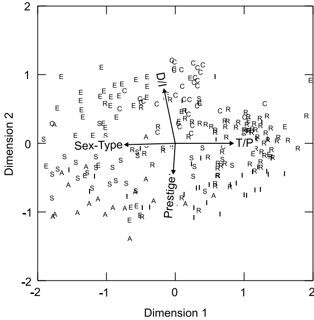
Fig. 5. Property vector fitting results for the Holland plane (dimensions one and two) of the rotated three-dimensional MDS solution, with occupations plotted by first-letter RIASEC code. D/I, Data/Ideas; T/P, Things/People.
